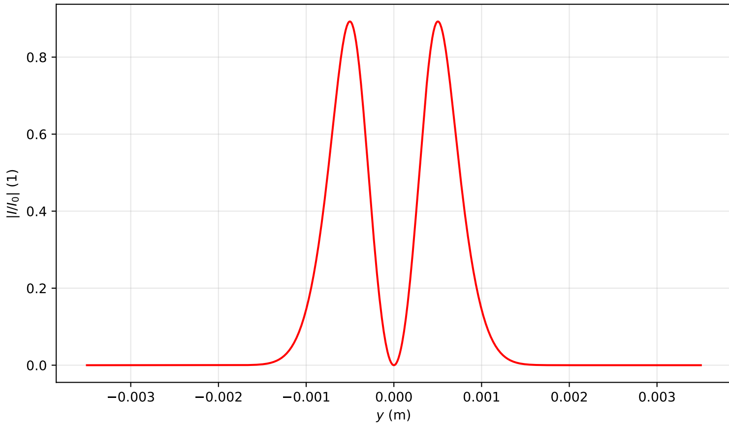
Intensity profile I(x=0, y, z=0.318)/I_0 , P_{in}=3.0P_{cr} , artificial time
